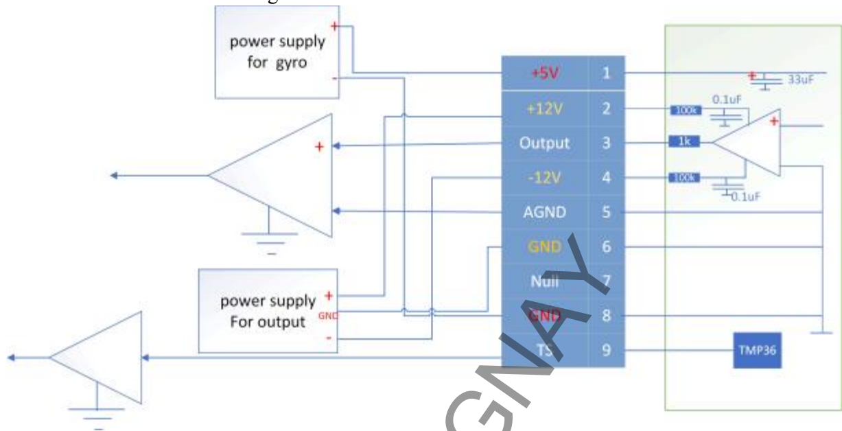
Fig 3 Electrical connection
